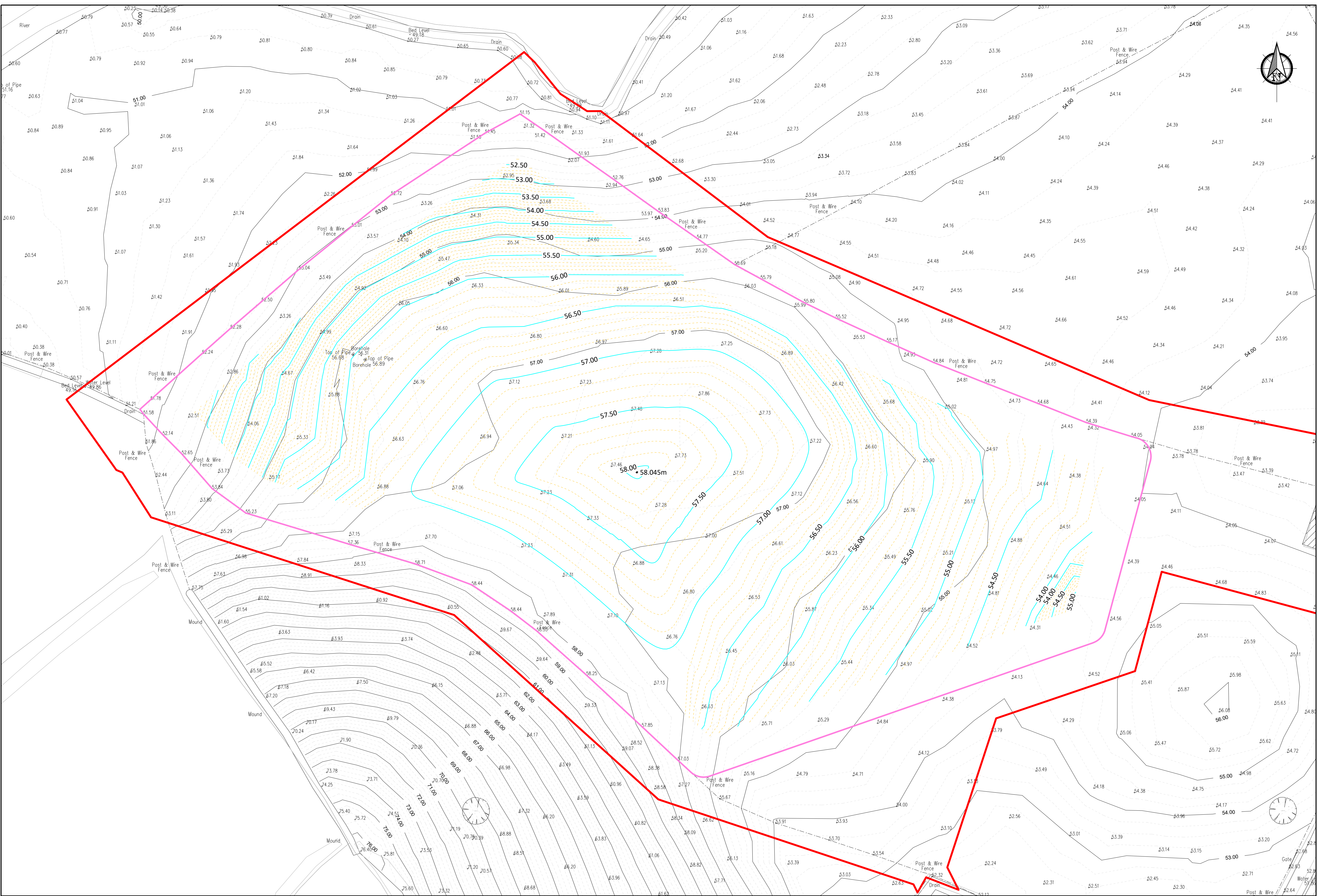
PLAN Scale 1:500
