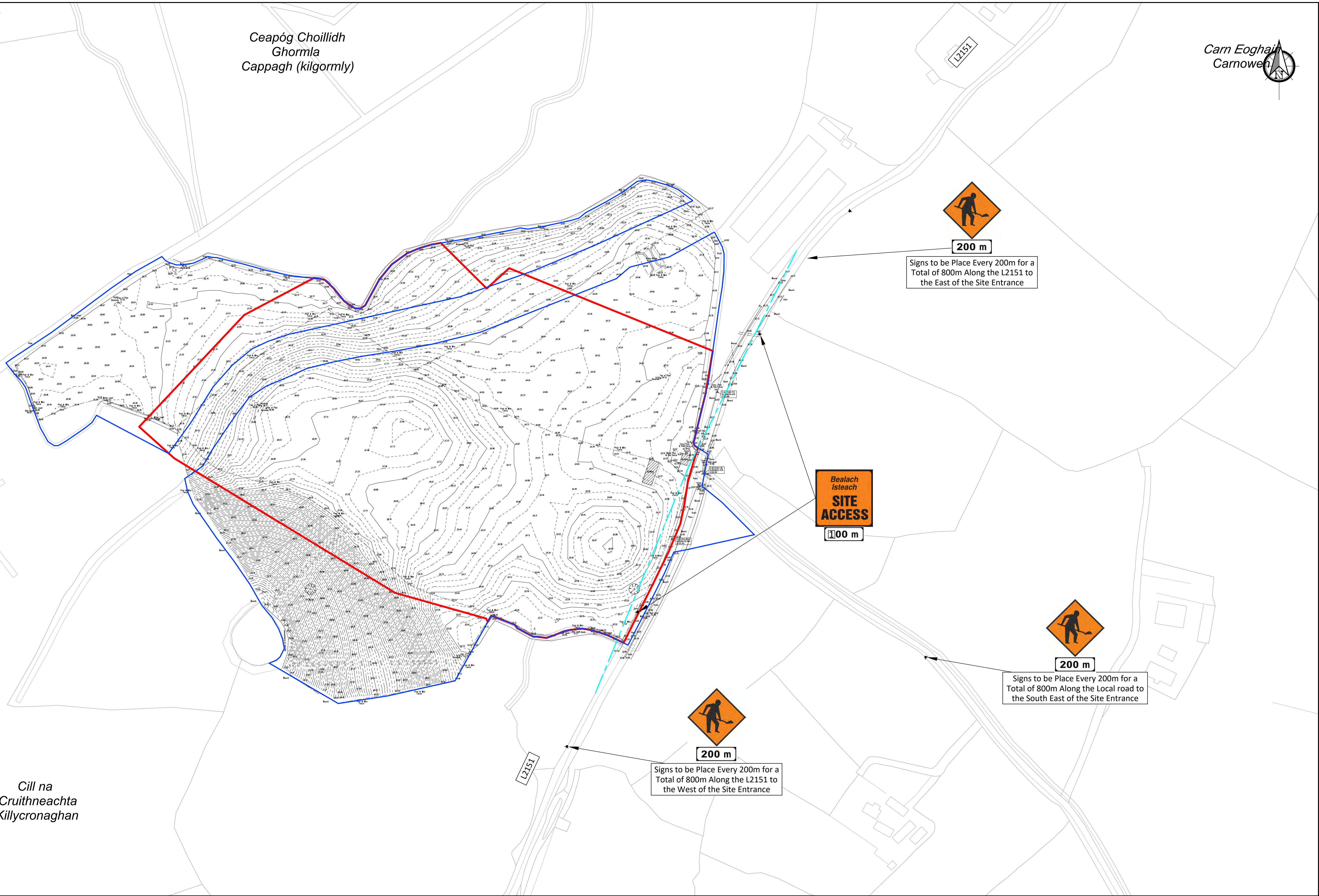
DRAFT PLANNING STAGE - TRAFFIC MANAGEMENT PLAN Scale 1:1250
