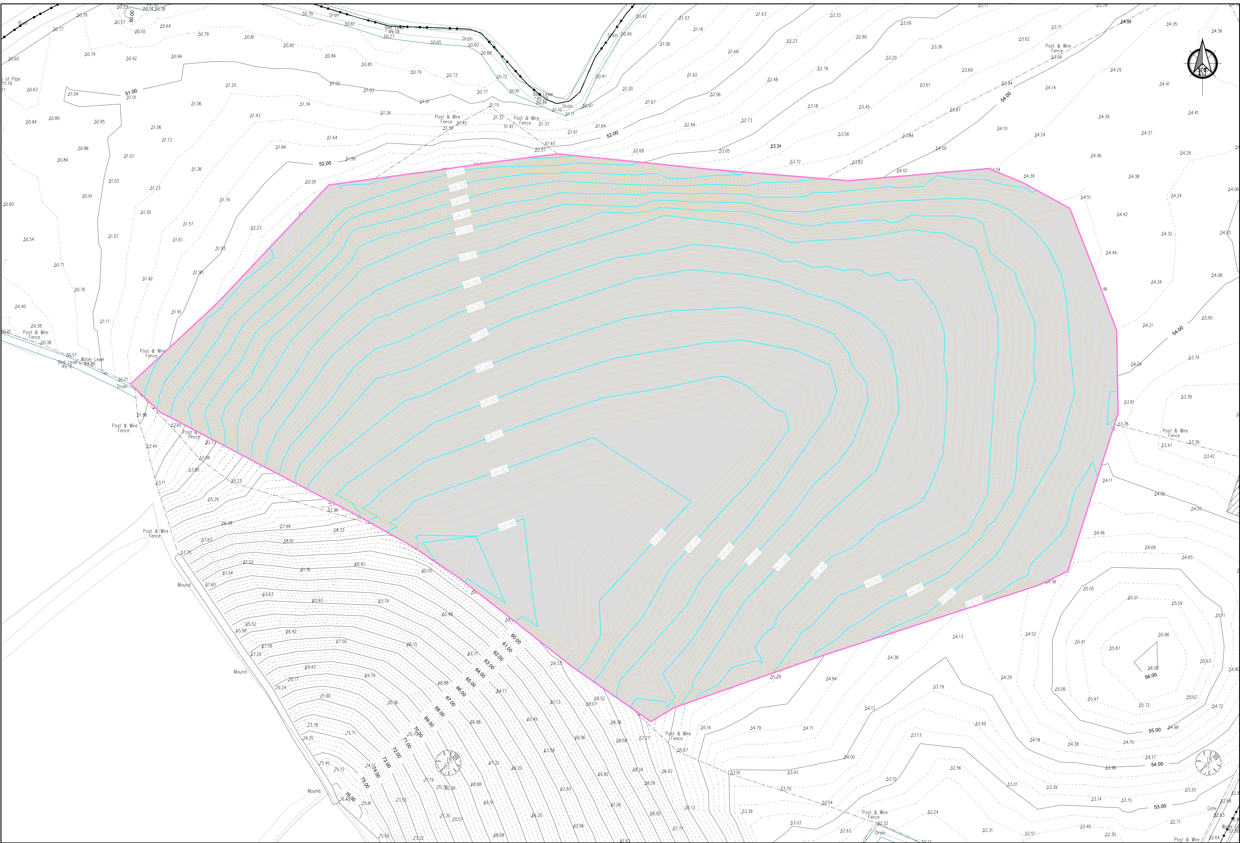
PLAN Scale 1:500
