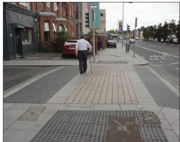
Figure 4.69: Example from Dorset Street, Dublin, where the carriageway has been raised and paved to slow turning vehicles and enhance the pedestrian crossing.
