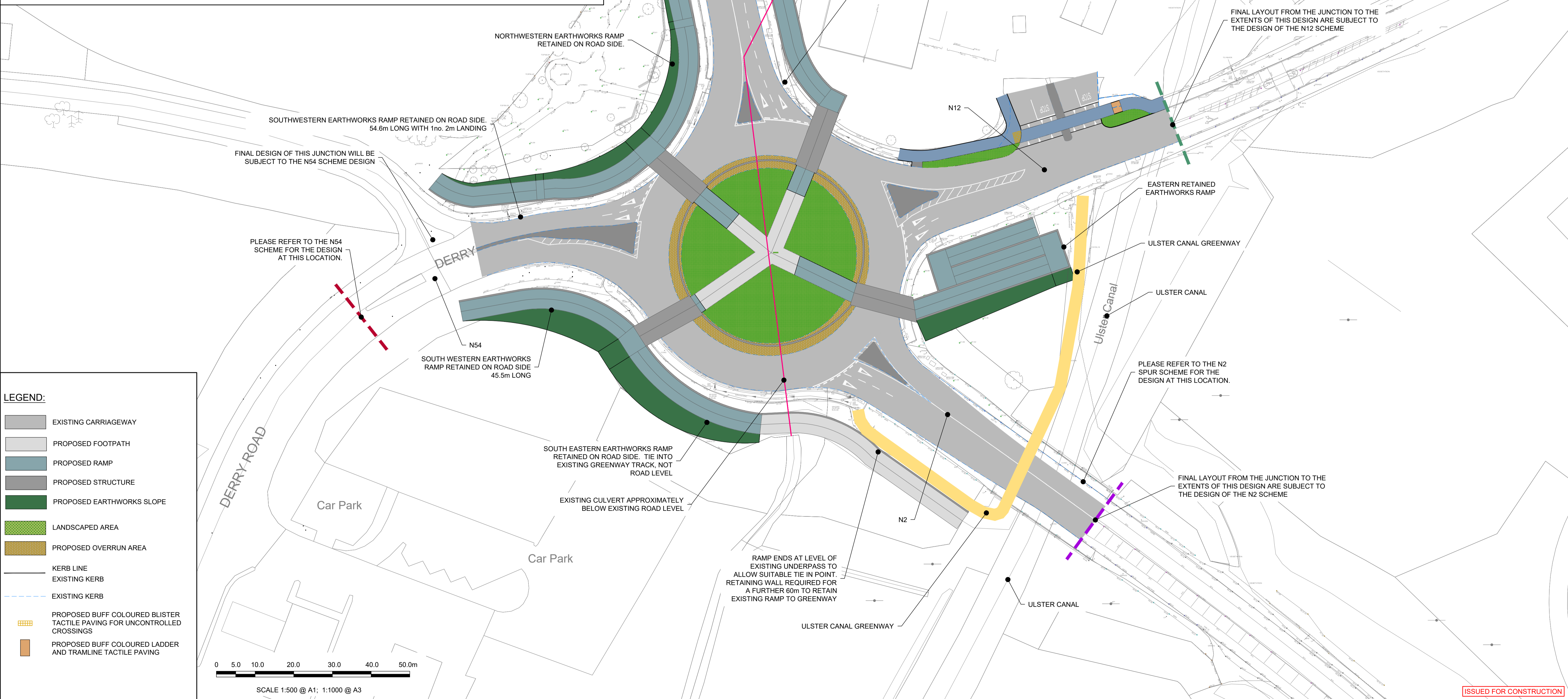
UNDERPASS CONCEPT LAYOUT
